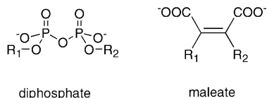
Figure 2. Comparison of diphosphate and maleates.
