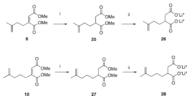
Scheme 4. Synthesis of flexible compounds. Reagents and conditions: (i) [(C 6 H 5 ) 3 PCu] 6 , toluene, 61% for 25 and 27 ; (b) LiOH, H 2 O/THF, quant for 26 and 28 .
