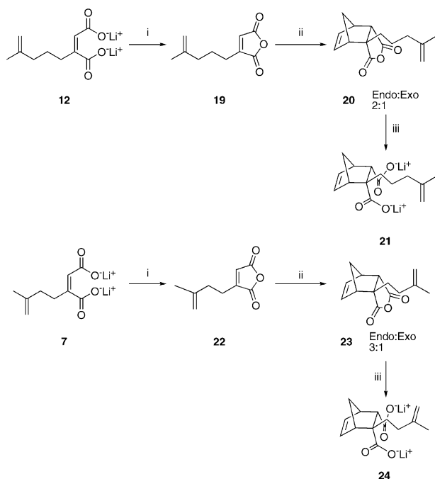
Scheme 3. Synthesis of rigid IPP analogues. Reagents and conditions: (i) HCl, Et 2 O, 80% for 19 and 76% for 22 ; (ii) cyclopentadiene, toluene, \Delta , 69% for 20 and 41% for 23 ; (iii) LiOH, H 2 O/THF, quant for 21 and 24 .
