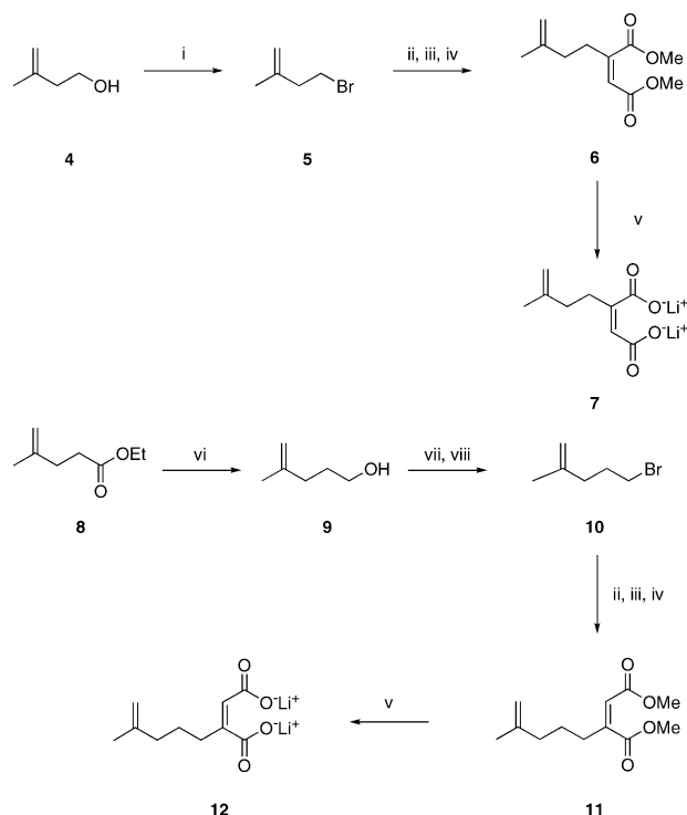
Scheme 1. Synthesis of IPP analogues. Reagents and conditions: (i) NBS, \text{PPh}_3 , \text{CH}_2\text{Cl}_2 , 16 h 40%; (ii) \text{Mg} , THF, \Delta , 2 h; (iii) \text{CuBr} \cdot \text{Me}_2\text{S} , THF, -40^\circ\text{C} , 2 h; (iv) DMAD, THF, -78^\circ\text{C} , 40% for 6 and 62% for 11 (over three steps); (v) \text{LiOH} , \text{H}_2\text{O}/\text{THF} , quant for 7 and 12 ; (vi) \text{LiAlH}_4 , THF, 88%; (vii) \text{TsCl} , \text{NEt}_3 , DMAP, \text{CH}_2\text{Cl}_2 ; (viii) \text{LiBr} , acetone, 18 h, 60% (over two steps).
