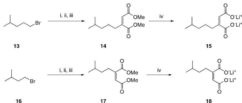
Scheme 2. Synthesis of saturated analogues. Reagents and conditions: (i) Mg, THF, \Delta , 2 h; (ii) CuBr·Me 2 S, THF, -40^{\circ}\text{C} , 2 h; (iii) DMAD, THF, -78^{\circ}\text{C} , 60% for 14 and 82% for 17 (over three steps); (iv) LiOH, H 2 O/THF, quant for 15 and 18 .
