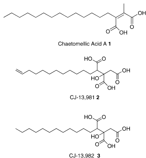
Figure 1. Polyanionic natural compounds.
