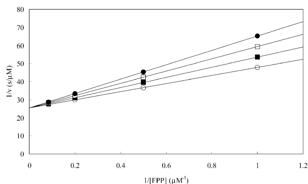
Figure 3. Inhibition of PFTase by compound 30 . Double-reciprocal plot with FPP as the varied substrate at fixed concentrations of 30 . Concentrations of analogue 30 were 100 (●), 200 (□), 300 (■), and 400 (○) \mu\text{M} . Dansyl-Gly-Val-Ile-Ala was held constant at 2.4 \mu\text{M} . PFTase (1.0 nM) was used to initiate reactions. Double-reciprocal plot was generated by fitting the data to the appropriate form of the Michaelis-Menten equation.
