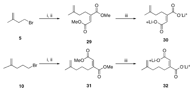
Scheme 5. Synthesis of trans IPP analogues. Reagents and conditions: (i) Mg, THF, \Delta , 2 h; (ii) DMAD, THF, -78^\circ\text{C} , 8% for 29 and 3% for 31 ; (d) LiOH, \text{H}_2\text{O}/\text{THF} , quantitative for 30 and 32 .
